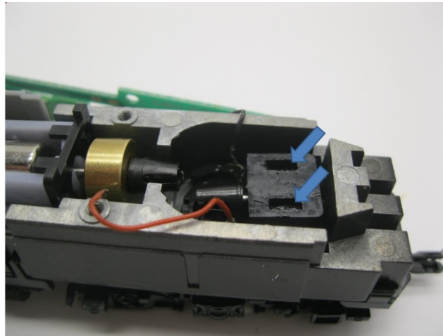
Klipps austragen Snap out the clips Clips losmaken
