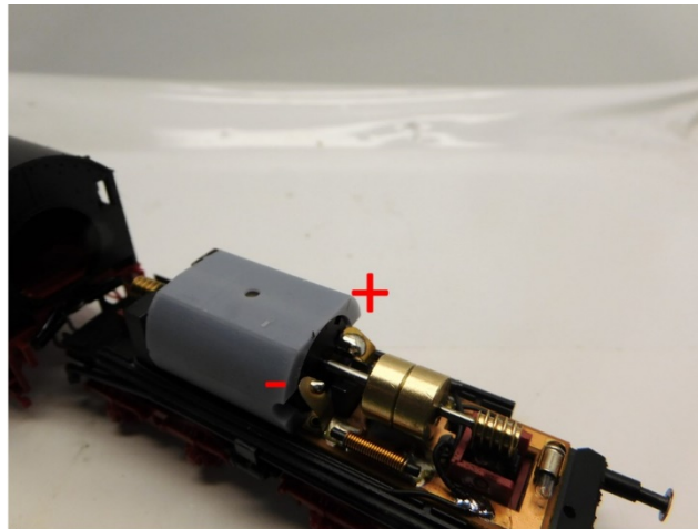
Kontakten löten Solder the contacts Soldeer de contacten
